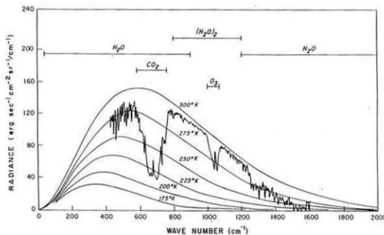
Fig. 4.1 The terrestrial infrared spectra and various absorption bands. Also shown is an actual atmospheric emission spectrum taken by the Nimbus 4 IRIS instrument near Guam at 15.1° N and 125.3° W on April 27, 1970.
