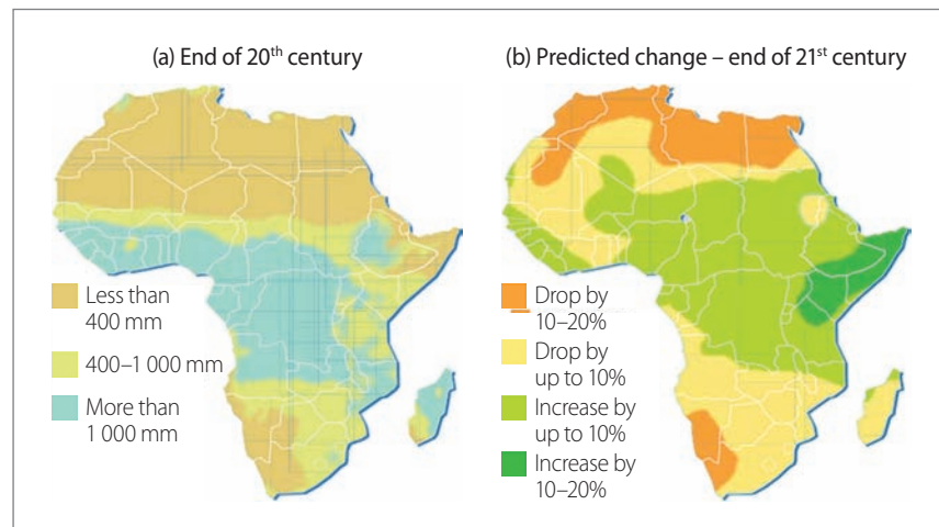
Figure 3.11 Precipitation change comparing end of 20th century with end of 21st century
