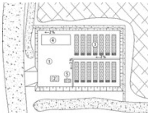
Figure II.1 Sketch map of COMPED Composting plant at Stung Meanchey
