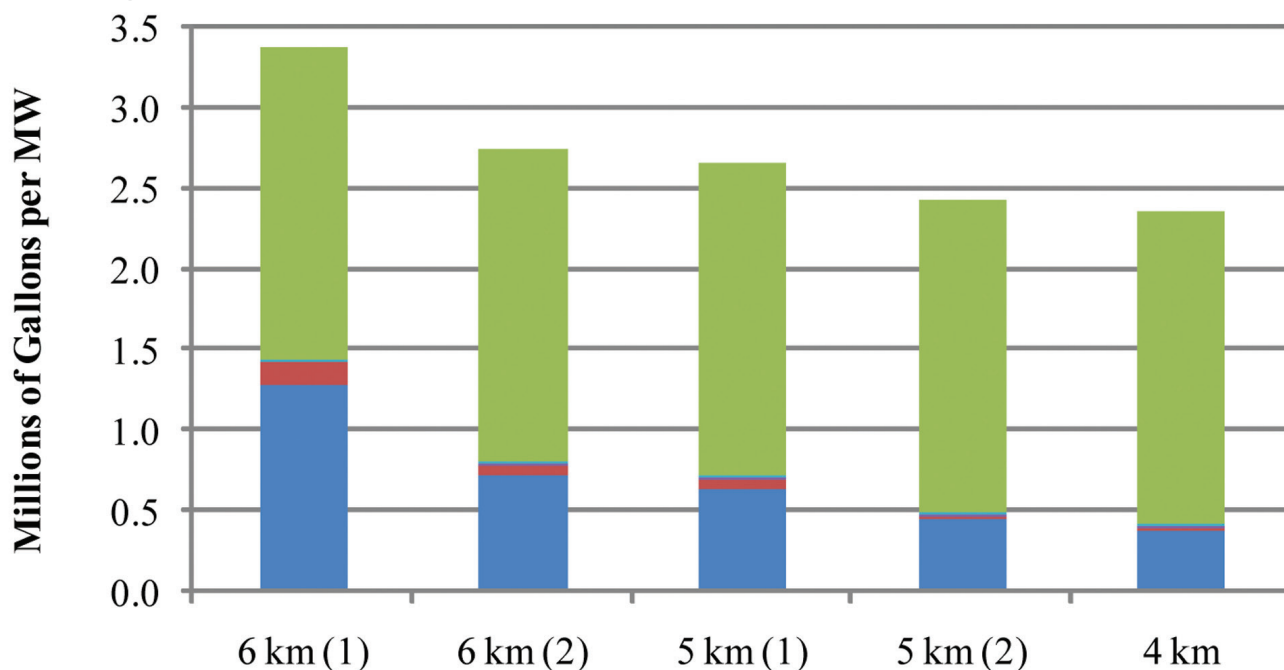
Figure 3 Hydraulic-Stimulation Water Use in Enhanced Geothermal Wells 57
