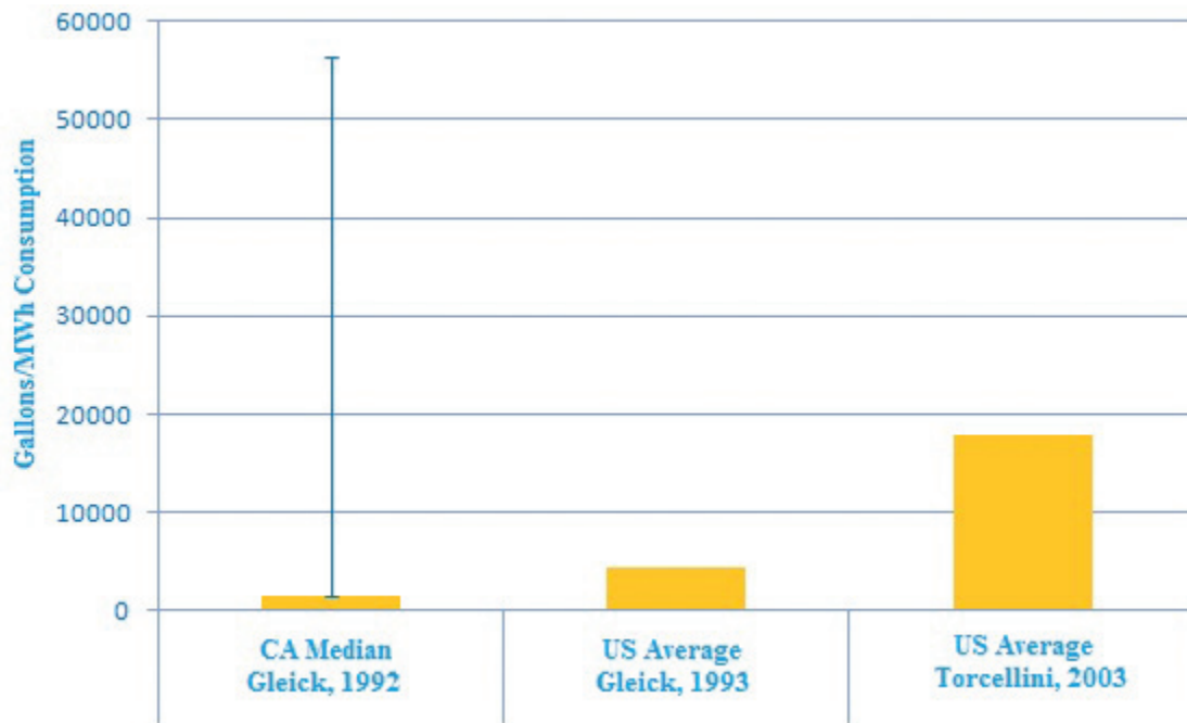
Figure 4 Hydropower Reservoir Evaporation Rates 61
