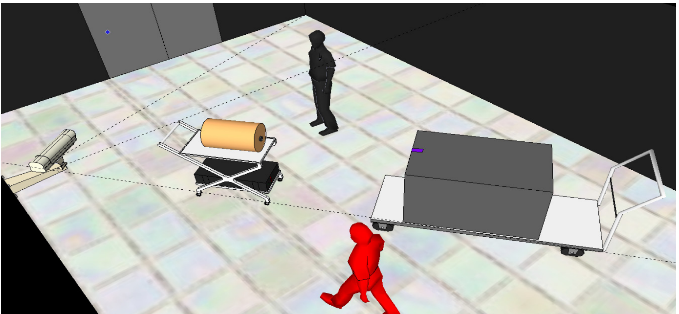
Figure 2 Example of 3D Model Design Support: Camera Placement and Field of View Refinements
