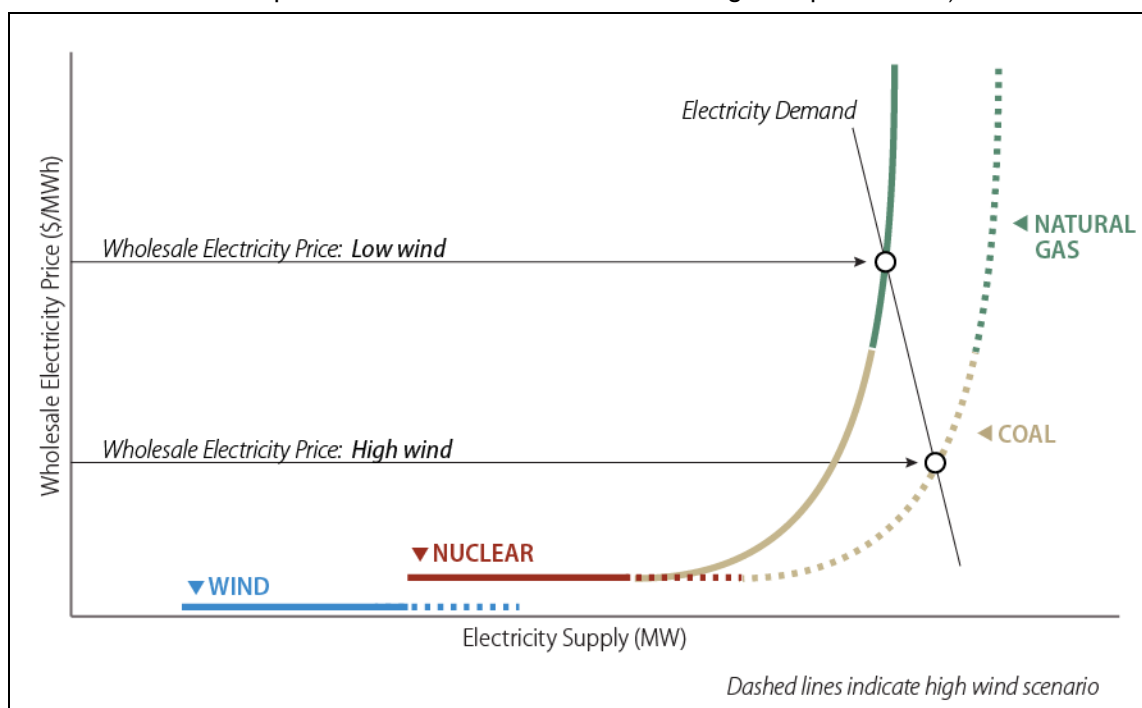
Figure 4. Illustration of Potential Wind Power Effects on Wholesale Electricity Prices
