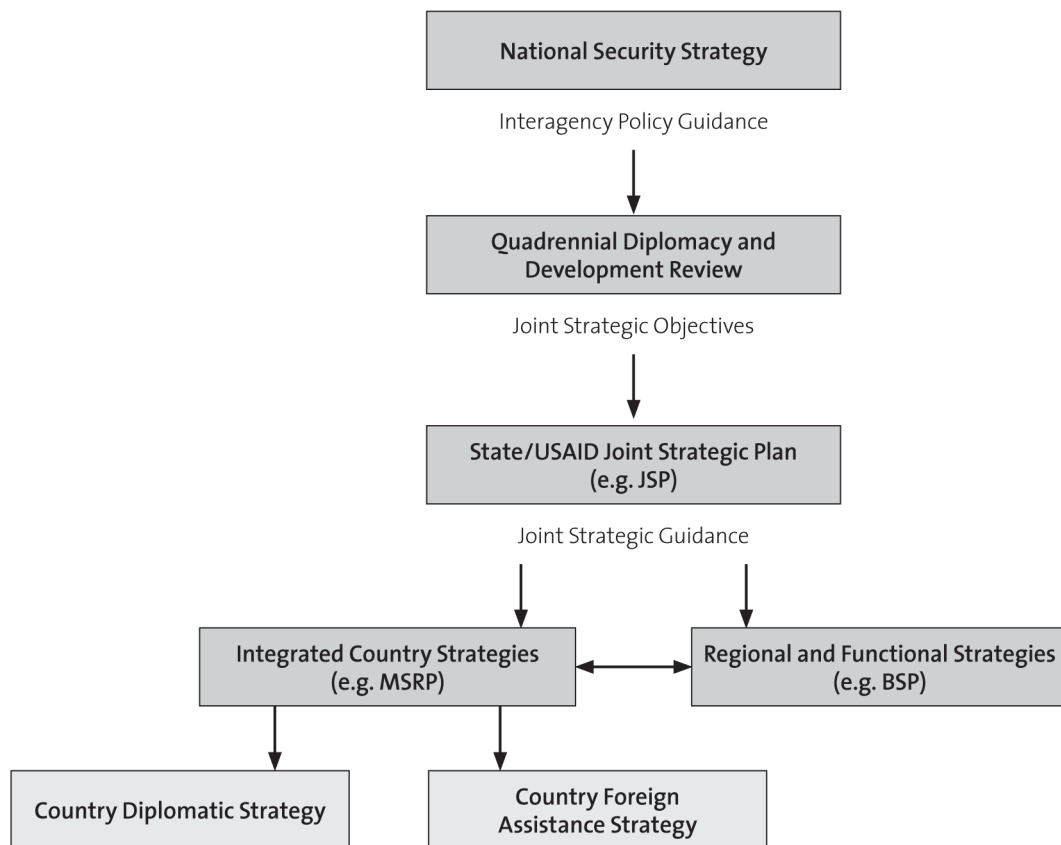
Figure 1: QDDR organisation
